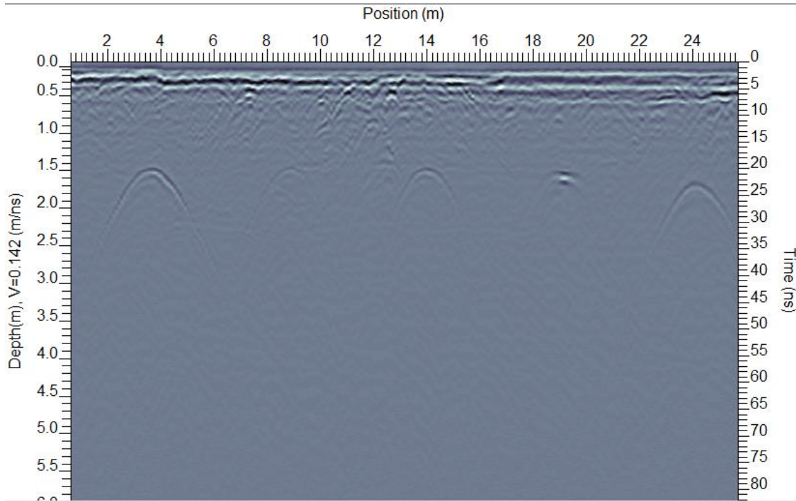
Figure 17: GPR line with no gain applied.
