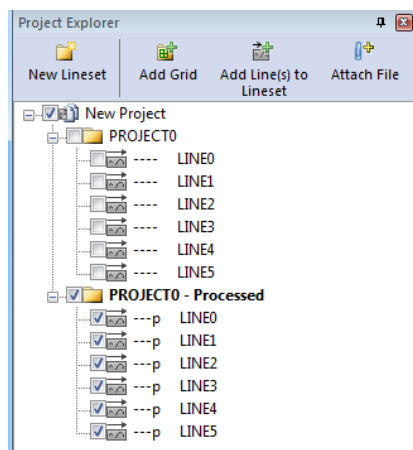
Figure 8: To process several GPR lines at once, check them in Project Explorer before selecting Process on the Toolbar or in the Tools menu.
