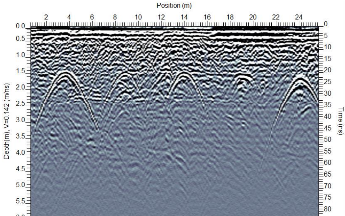
Figure 19: GPR line with a constant gain of 100 applied.
