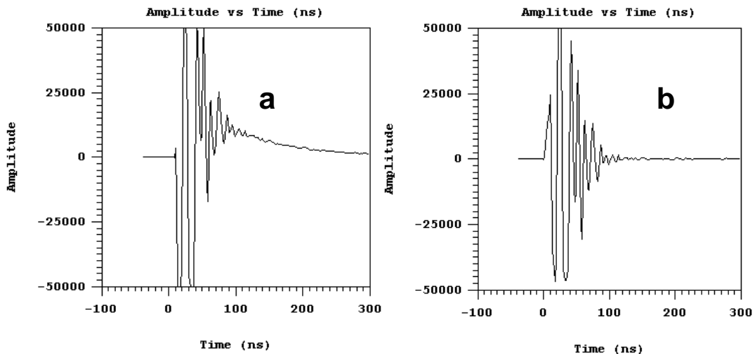
Figure 13: (a) Raw GPR trace with WOW. (b) GPR Trace with WOW removed using DEWOW.
