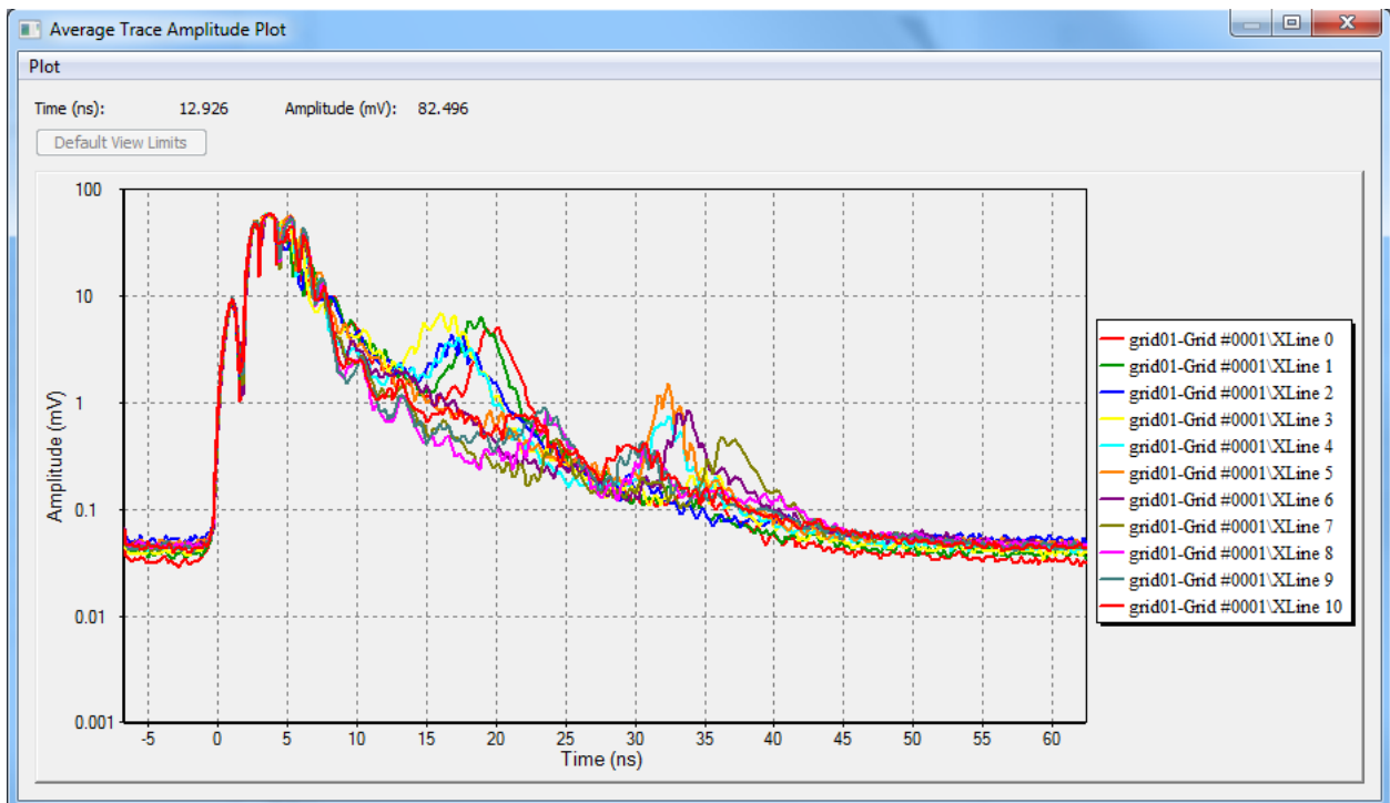
Figure 2: Average Trace Amplitude Plot
