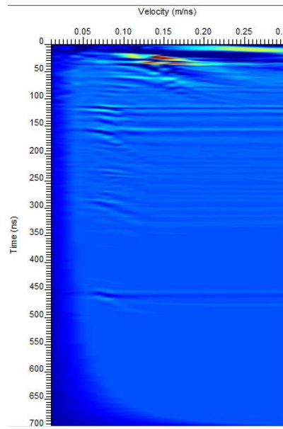
Analyzed CMP data – Auto gain
