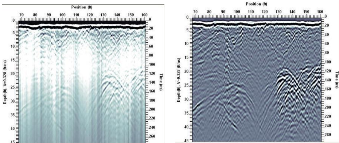
Figure 14: (Left) Raw GPR line with WOW. (Right) GPR line with WOW removed using DEWOW.
