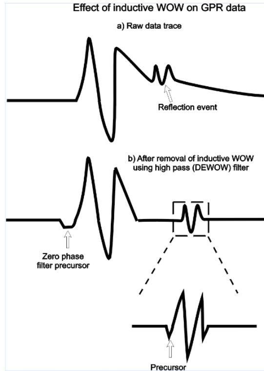
Figure 15: DEWOW artifacts: signal pre-cursor.
