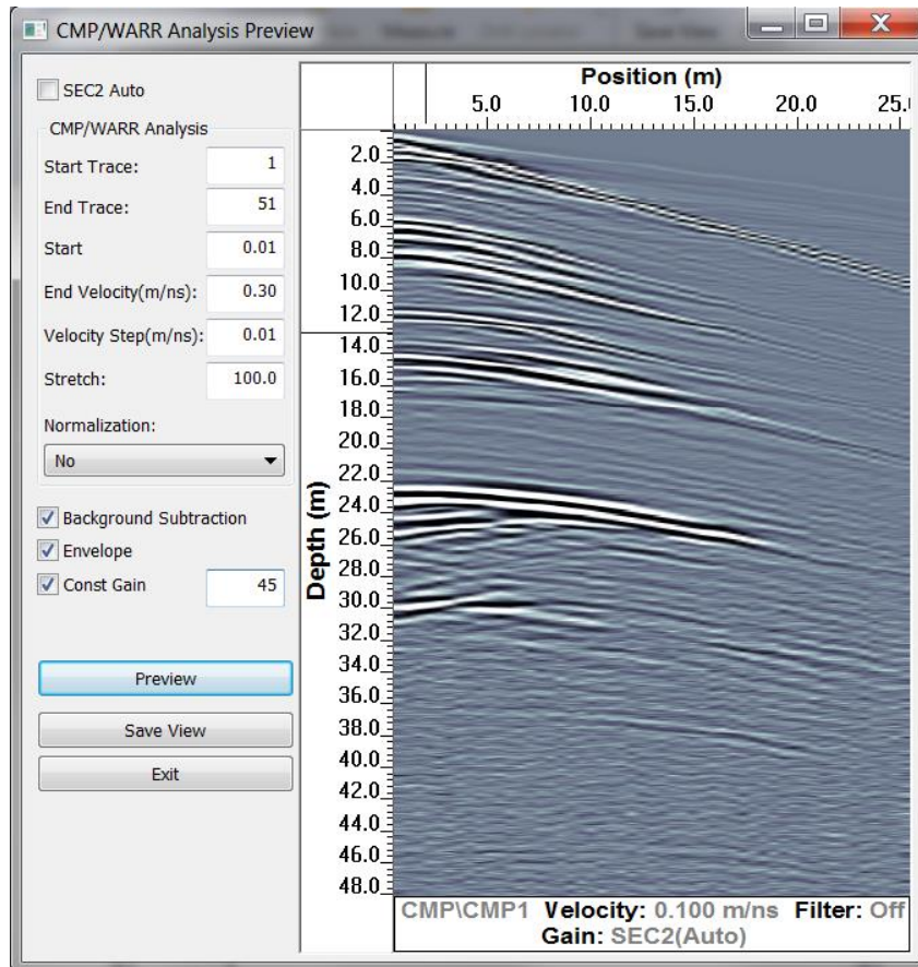
Figure 5: CMP Analysis dialog
