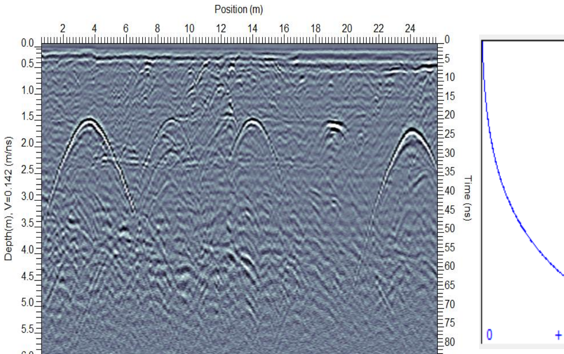
Figure 20: GPR line with an SEC2 gain applied and the SEC2 gain function on the right. This type of gain is the closest to physical reality because it compensates for the attenuation of the signal with depth.
