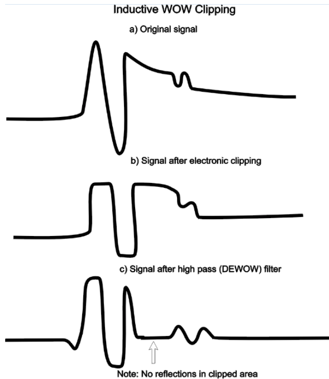
Figure 16: DEWOW artifacts: electronic clipping
