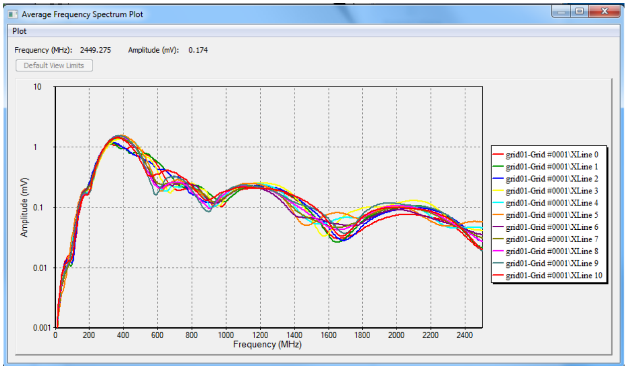
Figure 3: Average Frequency Spectrum Plot
