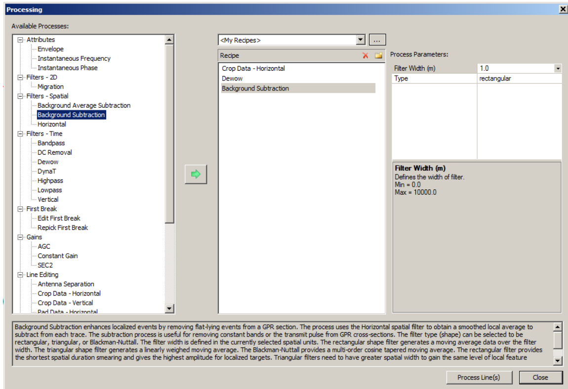
Figure 10: Processes added to the Recipes pane.
