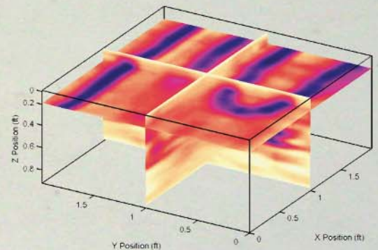
Locating radiant heating tubes
